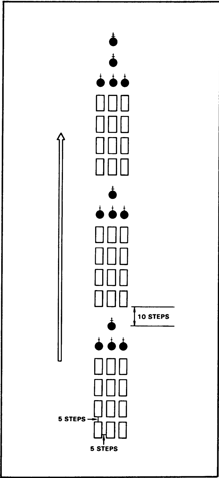
Figure D-2. Column of Masses
