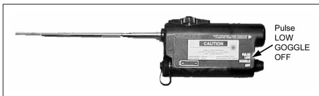
Figure 2-40. Borelight with a 5.56-mm mandrel.
