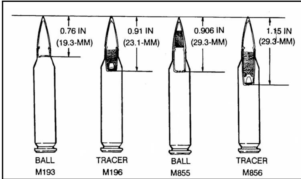
Figure 5-32. Projectile differences.
